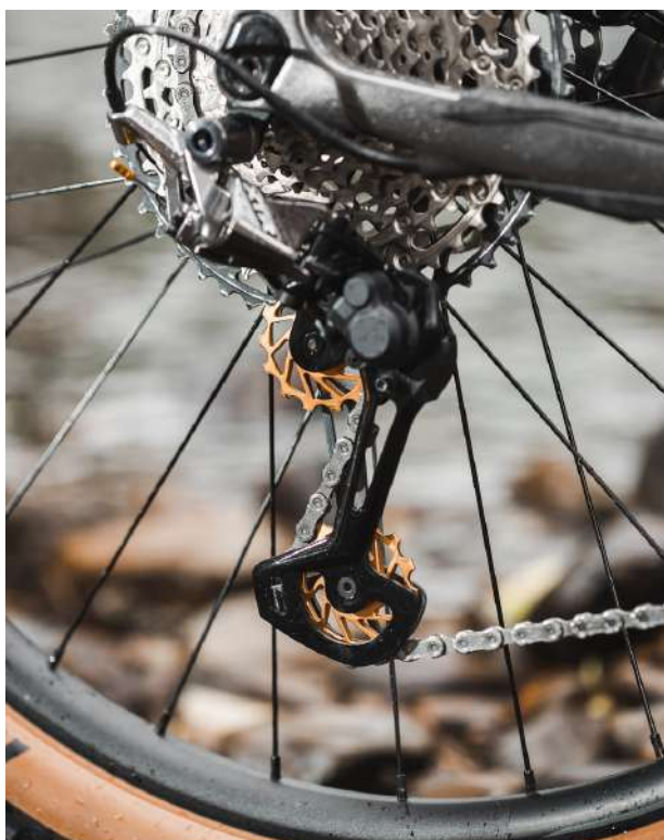
CERAMIC PULLEY WHEELS
